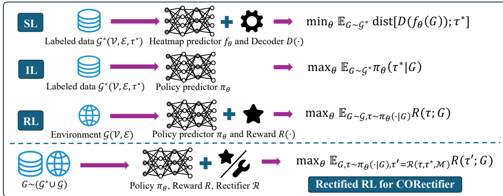
Figure 5: Mainstream NCO learning paradigms. SL minimizes the distance between model-predicted heatmaps and ground-truth matrices; IL and RL maximize the likelihood of expert trajectories or expected reward, respectively; Rectified RL aims to regularize exploration in RL via rectifiers \mathcal{R} .
