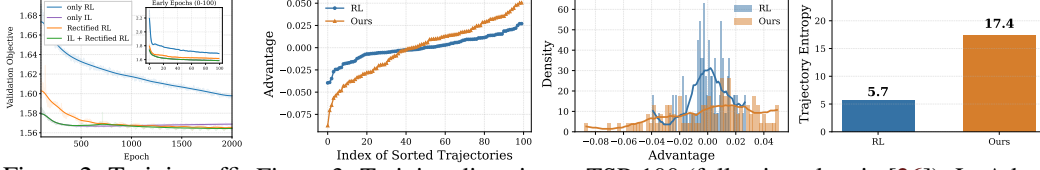
Figure 2: Training efficiency on ATSP-50. Figure 3: Training diversity on TSP-100 (following plots in [26]). L: Advantage separation. M: Advantage scale distribution. R: Trajectory entropy.
