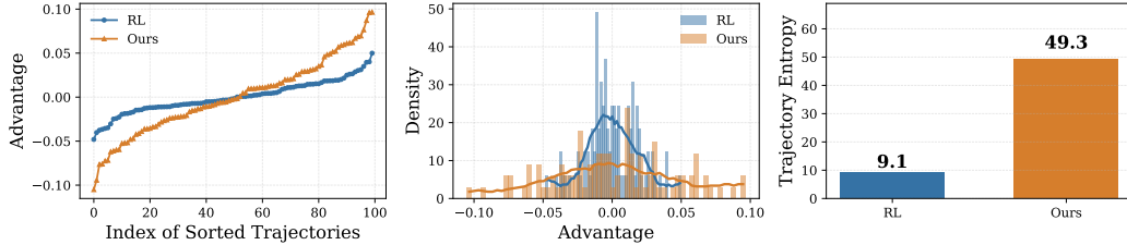
Figure 11: Exploration diversity on CVRP-100. Left: Advantage separation. Mid: Advantage scale distribution. Right: Trajectory entropy.
