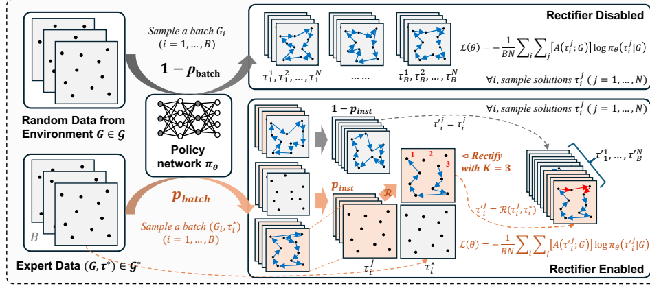
Figure 1: RRL stage of CORectifier. In general, B -sized batches are sampled from labeled data with prob. p_{\text{batch}} , and for each, N tours are sampled, of which a p_{\text{inst}} fraction undergo rectification if enabled. A(\cdot) : the advantage function; K : the (varying) rectified segment length.
