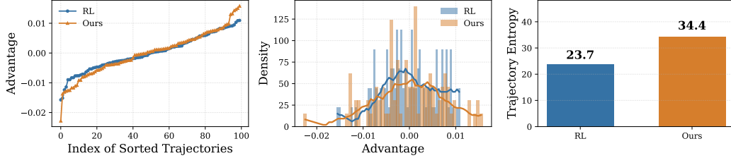
Figure 10: Exploration diversity on ATSP-100. Left: Advantage separation. Mid: Advantage scale distribution. Right: Trajectory entropy.
