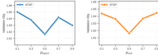
Figure 7: Effect of p_{\text{batch}} and p_{\text{inst}} on MatNet (for ATSP).
