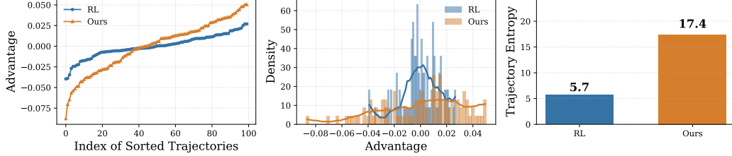
Figure 9: Exploration diversity on TSP-100. Left: Advantage separation. Mid: Advantage scale distribution. Right: Trajectory entropy.
