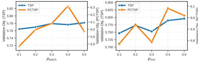
Figure 8: Effect of p_{batch} and p_{inst} on POMO (for TSP) and AM (for PCTSP).
